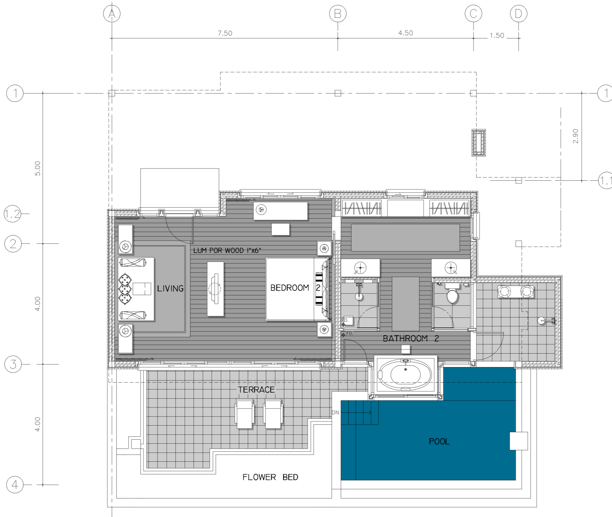
PROJECT : PARESA RESORT HOTEL LOWER FLOOR ( ARCH. 2 nd FL. ) FURNITURE LAYOUT PLAN
